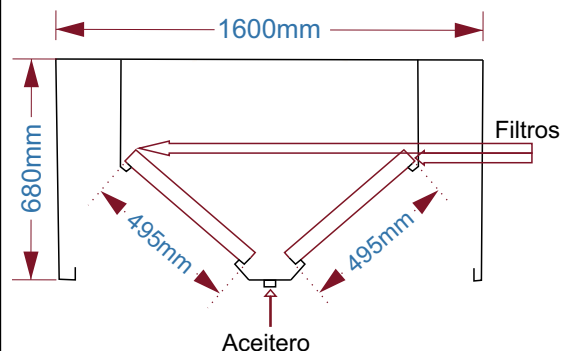
CAMPANA CENTRAL RECTA
